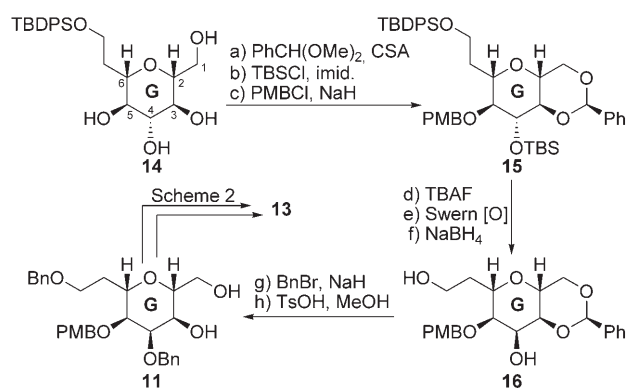
Scheme 3. Alternate construction of G ring system 13 . Reagents and conditions: a) PhCH(OMe) 2 (1.5 equiv), CSA (0.02 equiv), 4-Å MS, CH 2 Cl 2 , 25°C, 2 h, 74%; b) TBSCl (2.0 equiv), imid. (3.0 equiv), DMF, 25°C, 18 h, 88%; c) PMBCl (10 equiv), TBAI (0.5 equiv), NaH (6.0 equiv), DMF, 25°C, 18 h, 80%; d) TBAF (5.0 equiv), THF, 25°C, 18 h, 83%; e) (COCl) 2 (5.0 equiv), DMSO (10 equiv), CH 2 Cl 2 , –78°C, 1 h; Et 3 N (20 equiv), 0°C, 30 min; f) NaBH 4 (2.2 equiv), MeOH, 0°C, 86% over two steps; g) BnBr (7.0 equiv), TBAI (0.2 equiv), NaH (5.0 equiv), DMF, 25°C, 18 h, 88%; h) TsOH (0.2 equiv), MeOH, 25°C, 18 h, 85%. TBDPS = tert -butyldiphenylsilyl, CSA = (±)-camphor-10-sulfonic acid, MS = molecular sieves, DMF = N,N -dimethylformamide, TBAI = tetra- n -butylammonium iodide, TBAF = tetra- n -butylammonium fluoride.
